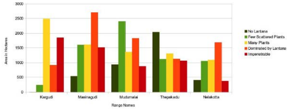
Lantana Infestation in Mudumalai Tiger Reserve
